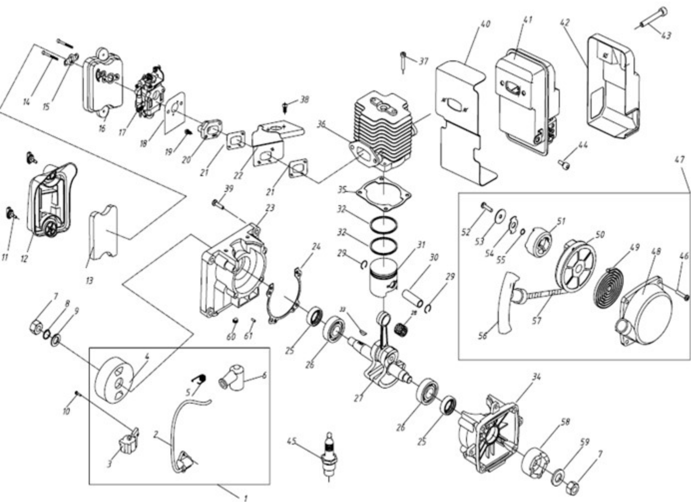
Fig. 1 ENGINE GROUP
