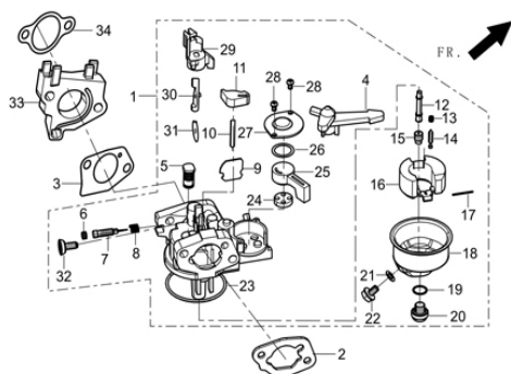
FIG.9 CARBURETOR ASSY. (E09)
