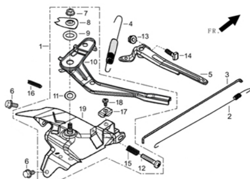
FIG.11 CONTROL ASSY, THROTTLE (E11)
