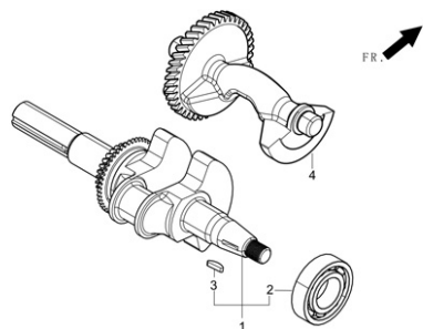
FIG.4 ROD,CRANKSHAFT CONNETING (E04)
