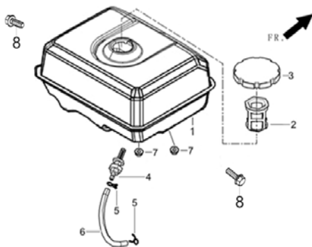
FIG.14 TANK ASSY, FUEL (F03)
