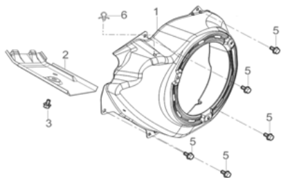
FIG.8 SHROUD / SHIELD,LOWER (E08)
