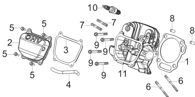
FIG.3 HEAD SUBASSEMBLY, CYLINDER / PLUG, SPARK (E03)
