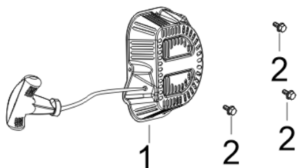
FIG.7 STARTER,RECOIL (E07)
