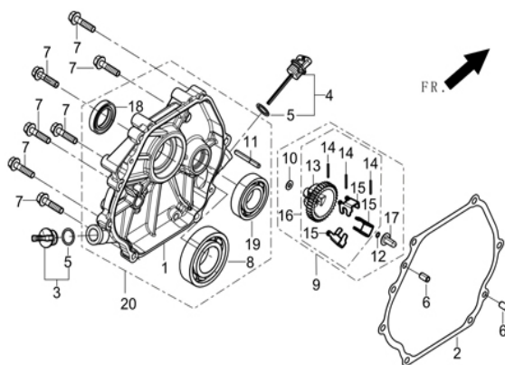
FIG.2 COVER SUBASSEMBLY, CRANKCASE / GEAR ASSY, GOVERNOR (E02)
