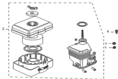
FIG.12 CLEANER, AIR 空滤器(F01)
