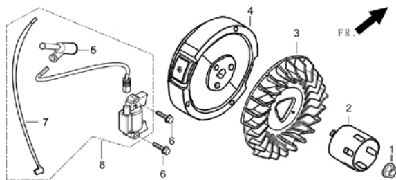
FIG.10 FLYWHEEL / IMPELLER / STARTER PULLEY / IGNITION COIL (E10)
